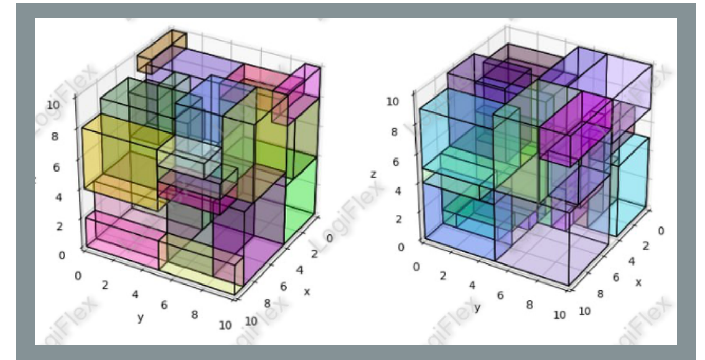
optimal algorithm
