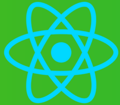
React
